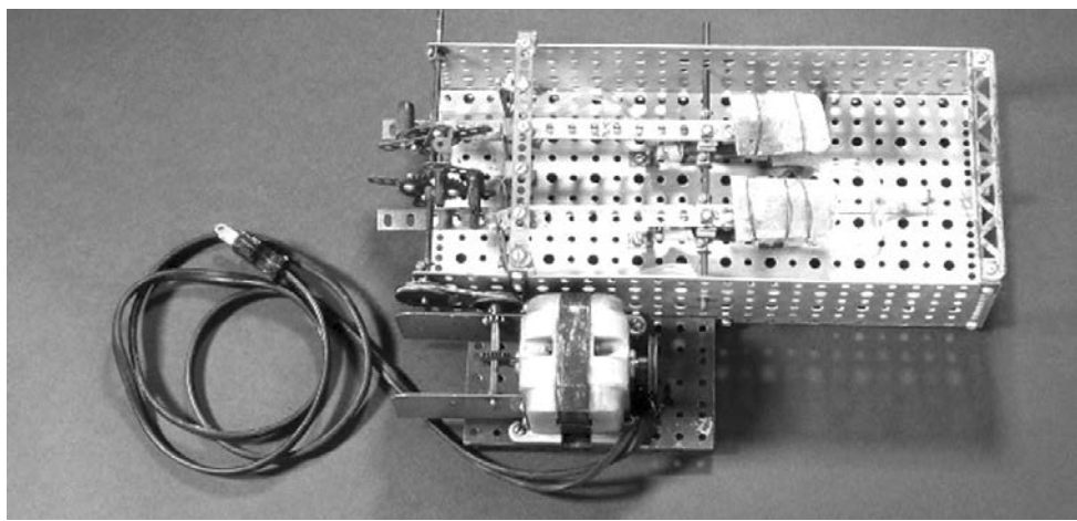
Above: William Sewell and William Glenn built this Erector artificial heart, called the Sewell heart pump, in 1949, using an Erector Set. This pump now resides in the National Museum of American History.
